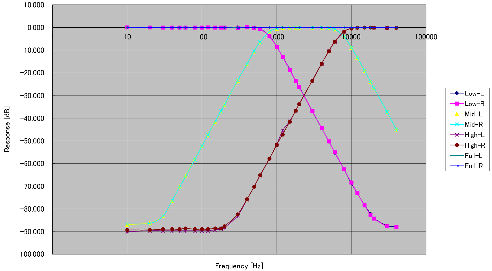
Frequency Response
